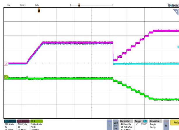
Figure 9. Soft Start into Heating Mode (VIN=3.3V with 5Ω load)
